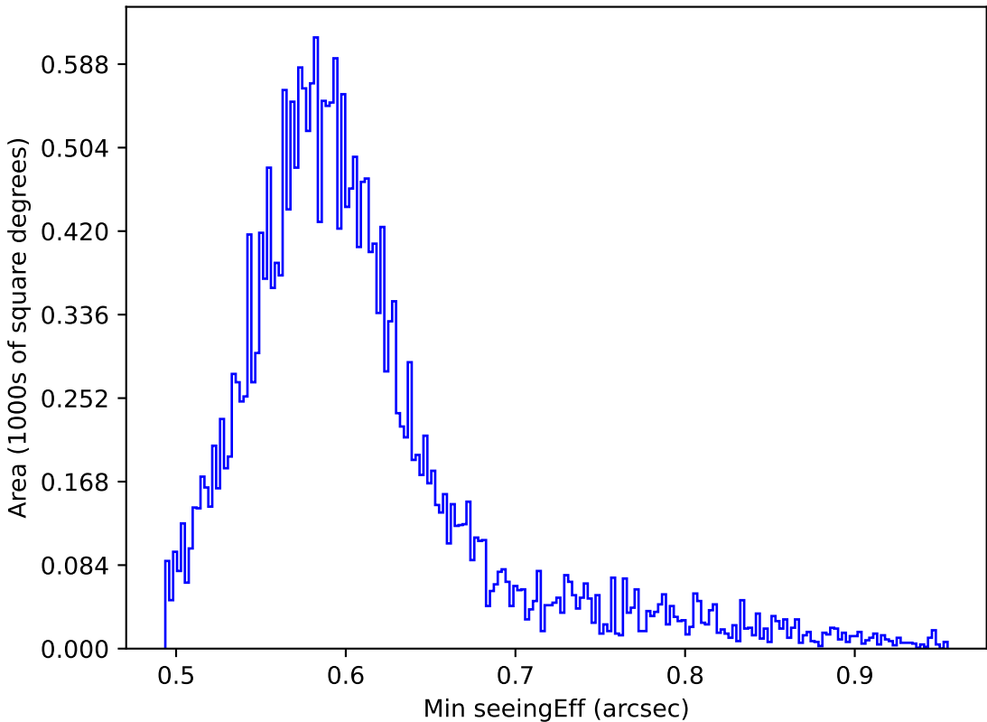
weather_cloudso31v3.4_10yrs All sky all bands: Min seeingEff
