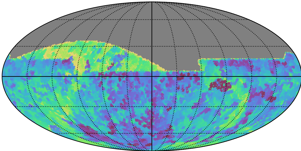
weather_cloudso31v3.4_10yrs All sky all bands: Min saturation_mag
