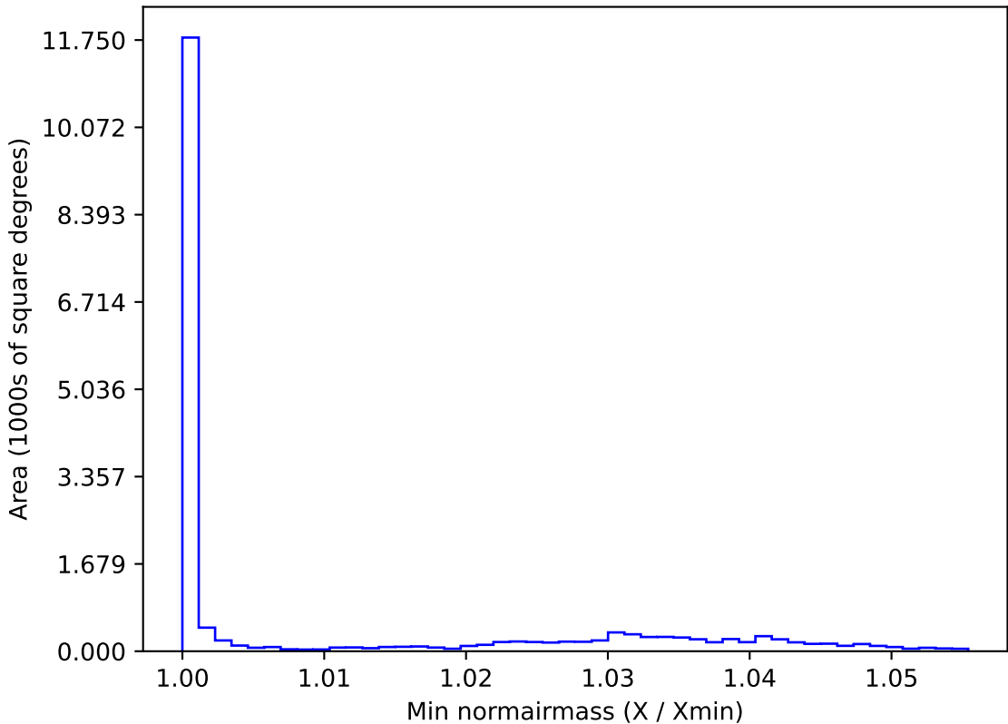
weather_cloudso31v3.4_10yrs WFD u band: Min normairmass
