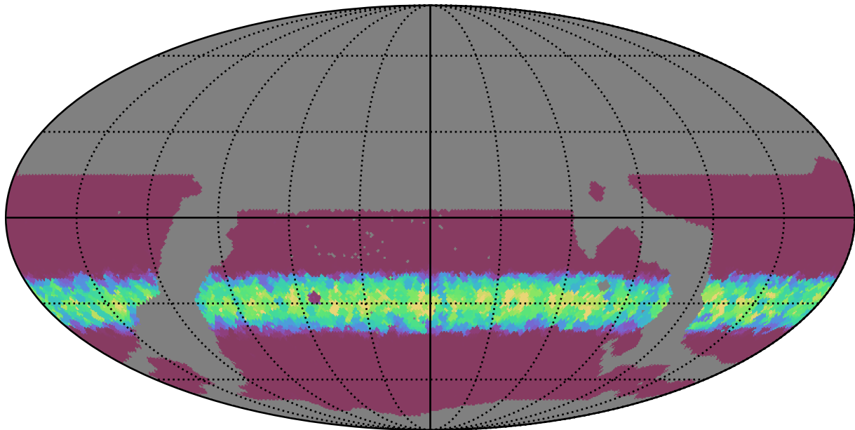
weather_cloudso31v3.4_10yrs WFD r band: Min normairmass
