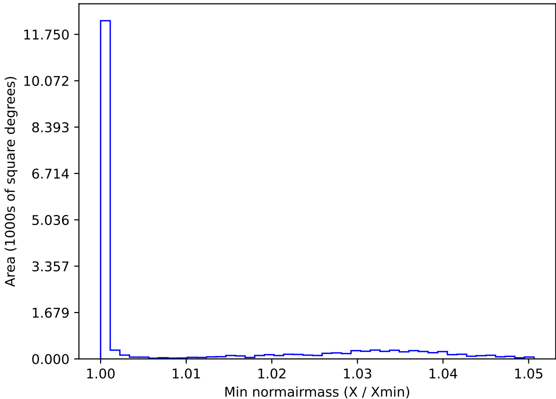
weather_cloudso31v3.4_10yrs WFD g band: Min normairmass
