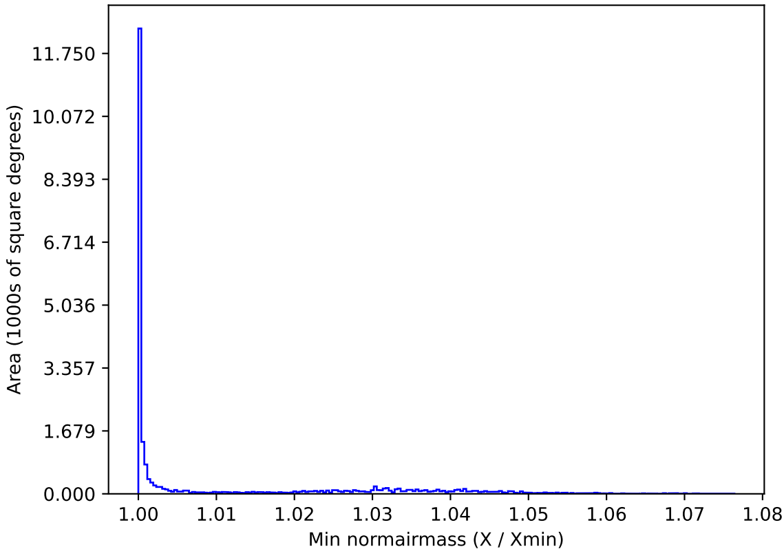
weather_cloudso31v3.4_10yrs All sky u band: Min normairmass
