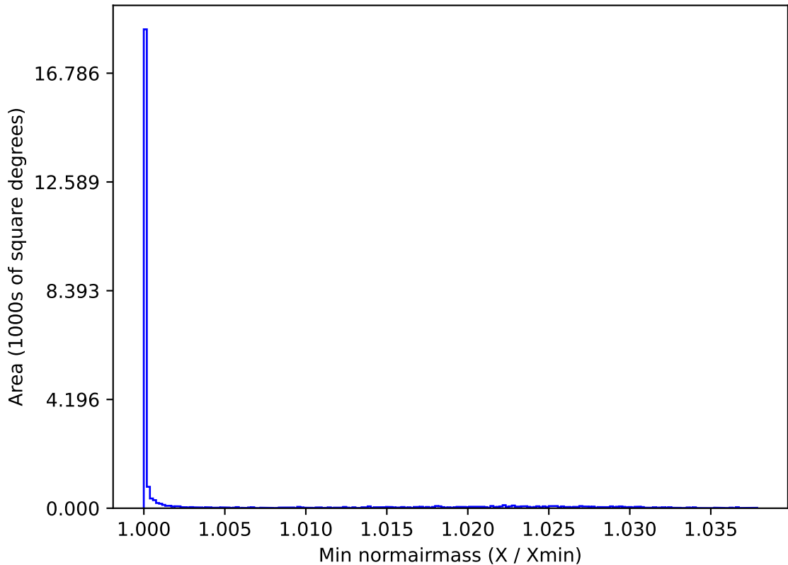
weather_cloudso31v3.4_10yrs All sky r band: Min normairmass
