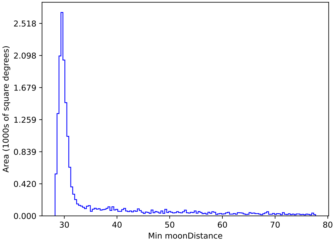
weather_cloudso31v3.4_10yrs WFD z band: Min moonDistance
