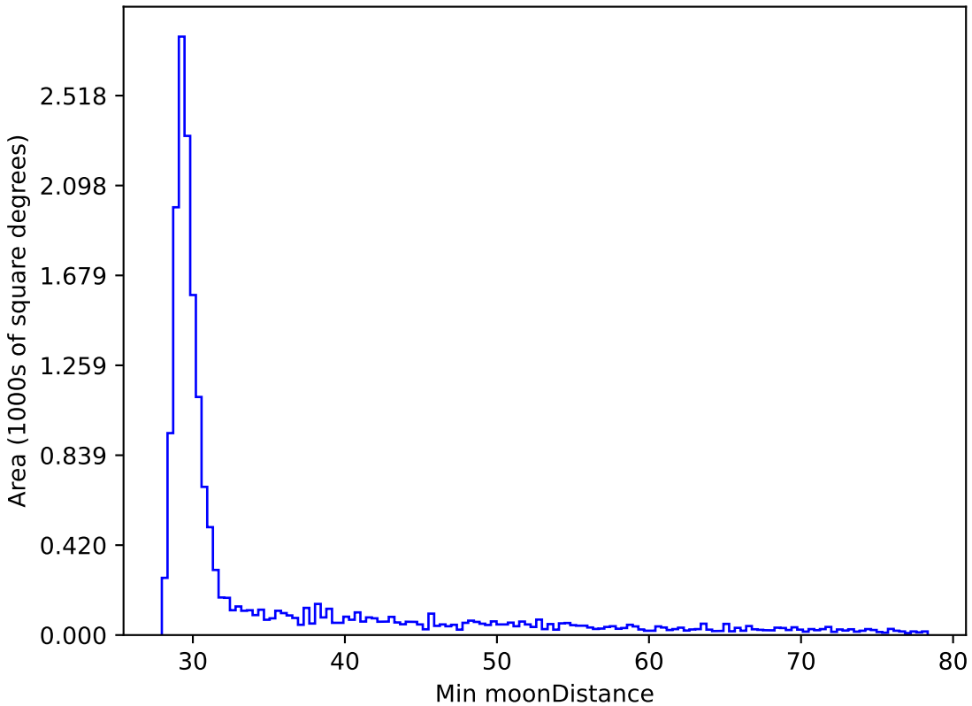
weather_cloudso31v3.4_10yrs WFD y band: Min moonDistance
