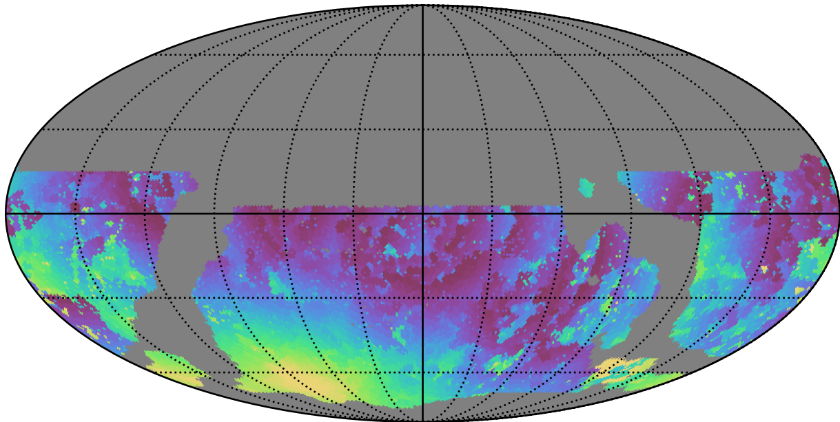
weather_cloudso31v3.4_10yrs WFD u band: Min moonDistance
