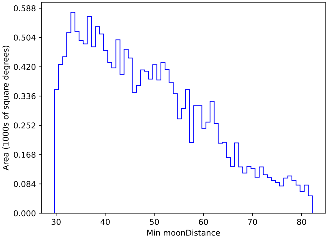
weather_cloudso31v3.4_10yrs WFD u band: Min moonDistance
