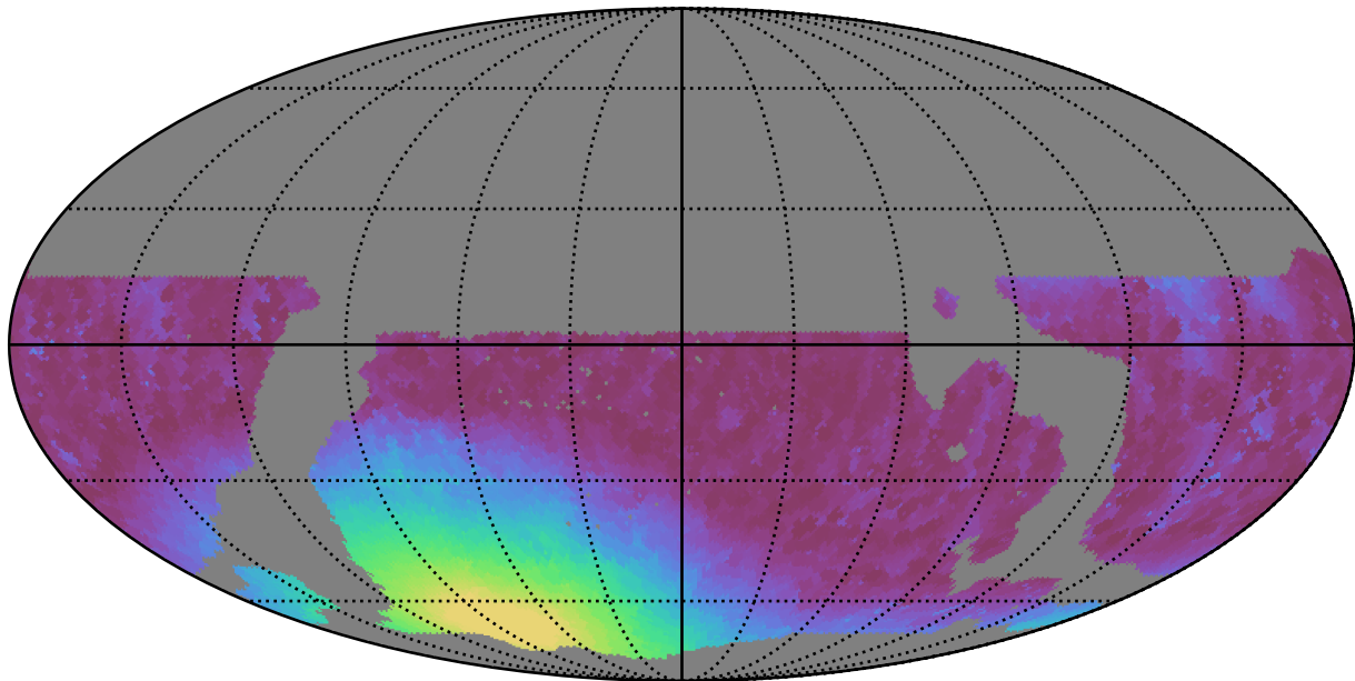
weather_cloudso31v3.4_10yrs WFD r band: Min moonDistance
