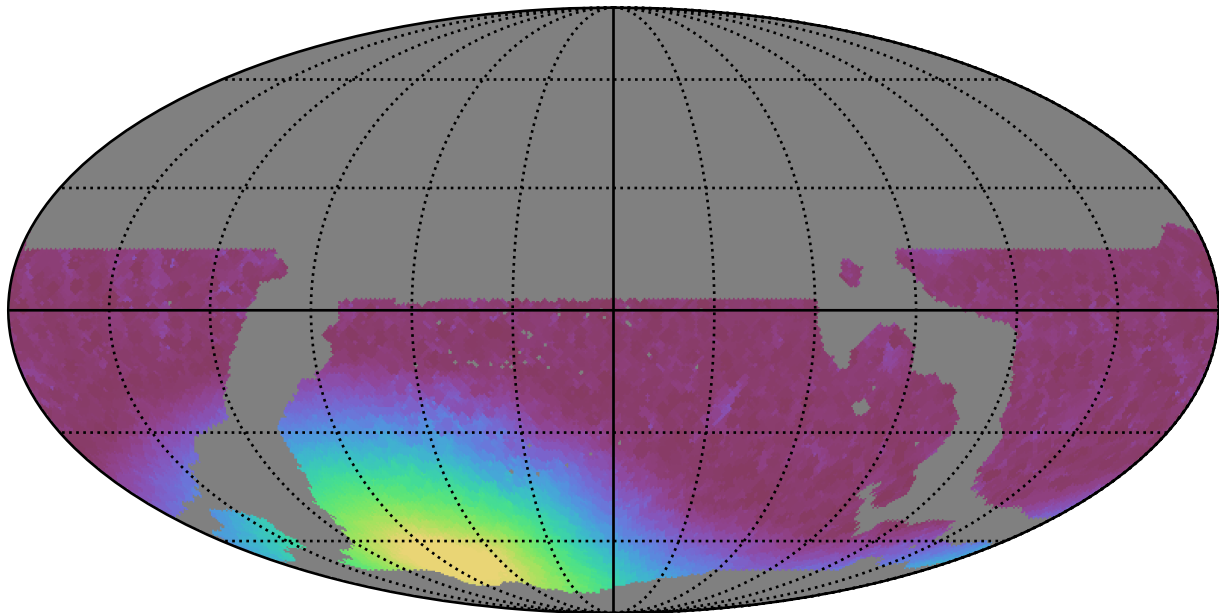
weather_cloudso31v3.4_10yrs WFD i band: Min moonDistance
