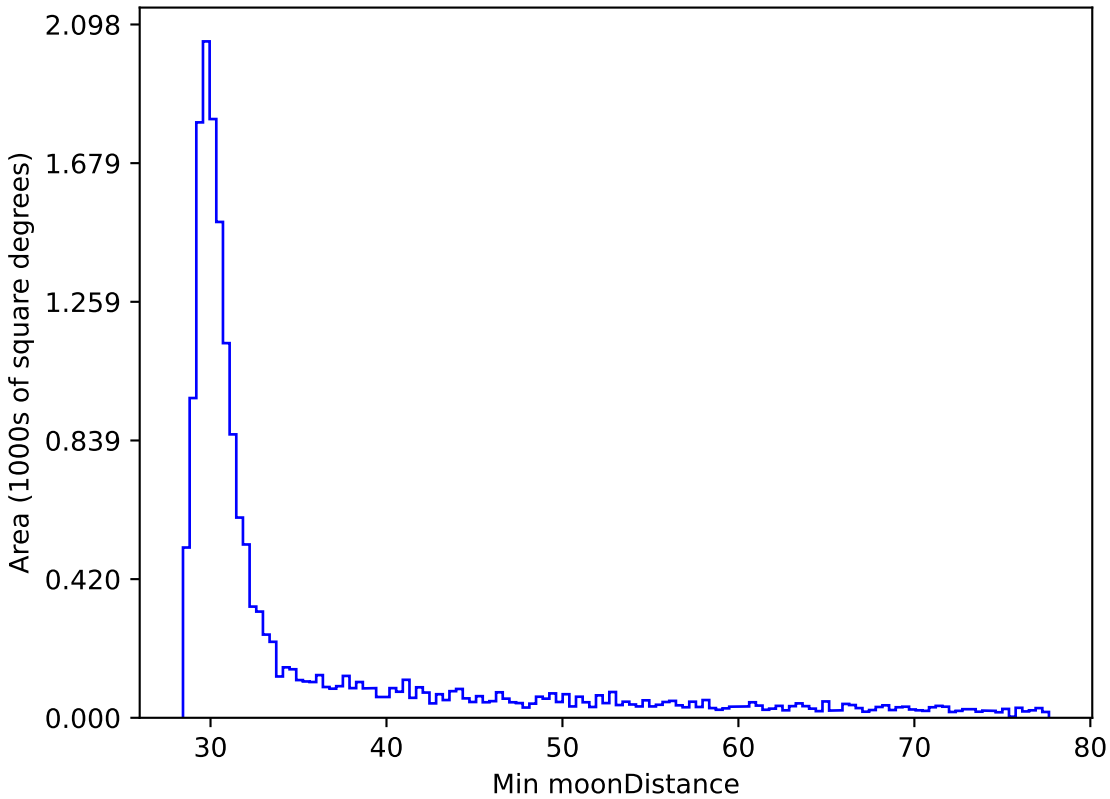
weather_cloudso31v3.4_10yrs WFD i band: Min moonDistance
