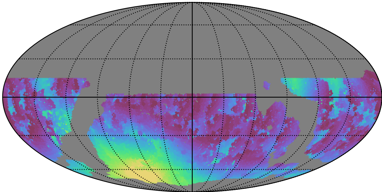
weather_cloudso31v3.4_10yrs WFD g band: Min moonDistance
