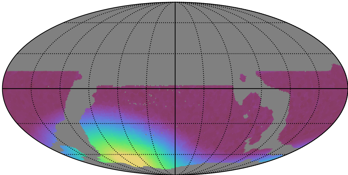
weather_cloudso31v3.4_10yrs WFD all bands: Min moonDistance
