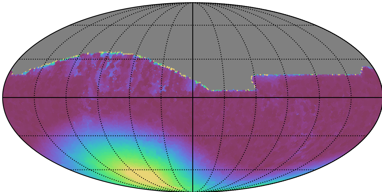
weather_cloudso31v3.4_10yrs All sky z band: Min moonDistance
