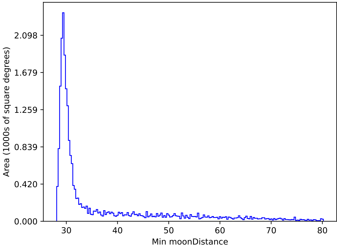
weather_cloudso31v3.4_10yrs All sky y band: Min moonDistance
