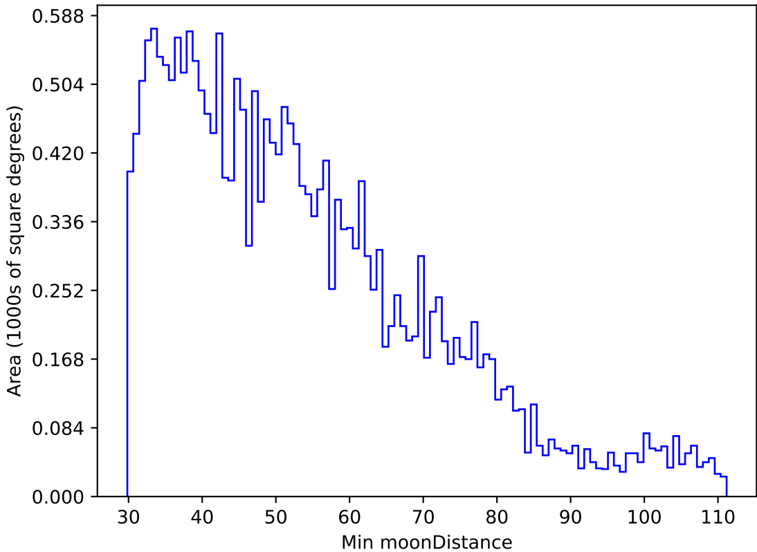
weather_cloudso31v3.4_10yrs All sky u band: Min moonDistance
