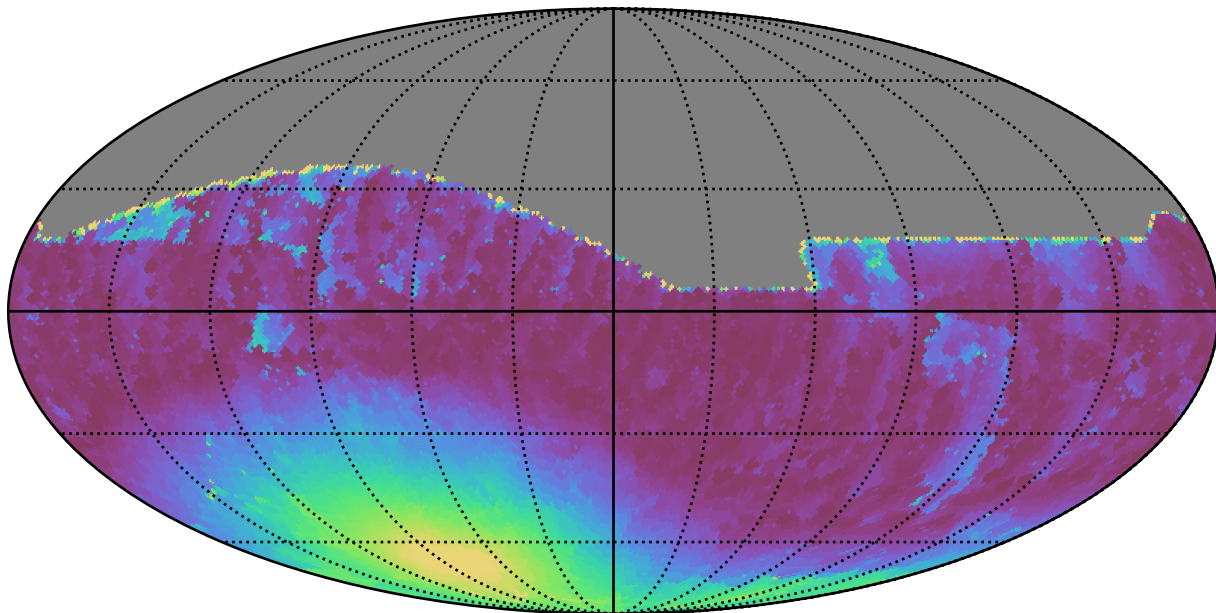
weather_cloudso31v3.4_10yrs All sky r band: Min moonDistance
