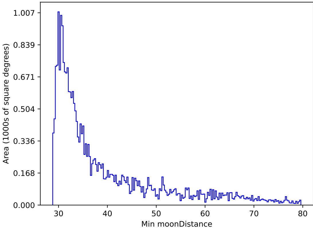
weather_cloudso31v3.4_10yrs All sky r band: Min moonDistance
