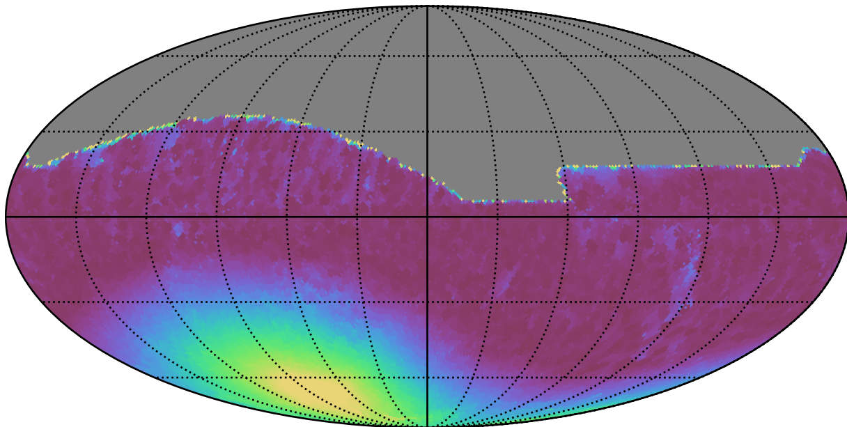
weather_cloudso31v3.4_10yrs All sky i band: Min moonDistance
