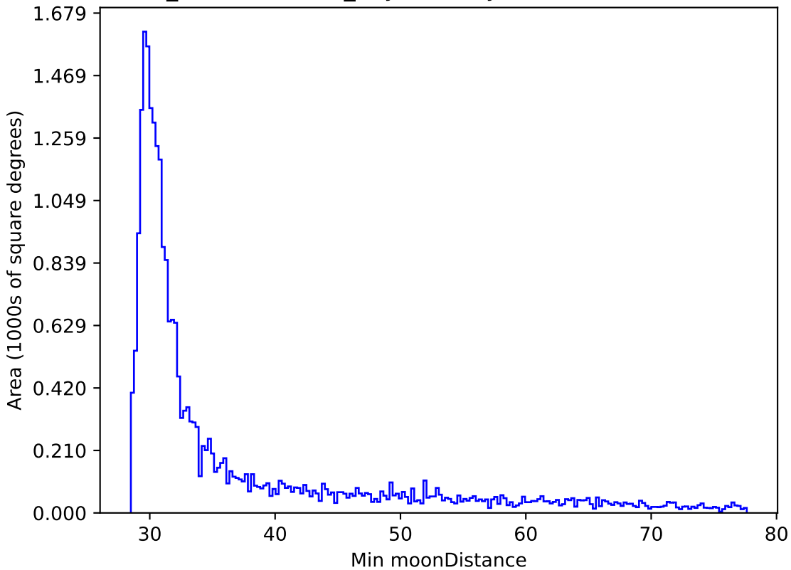
weather_cloudso31v3.4_10yrs All sky i band: Min moonDistance
