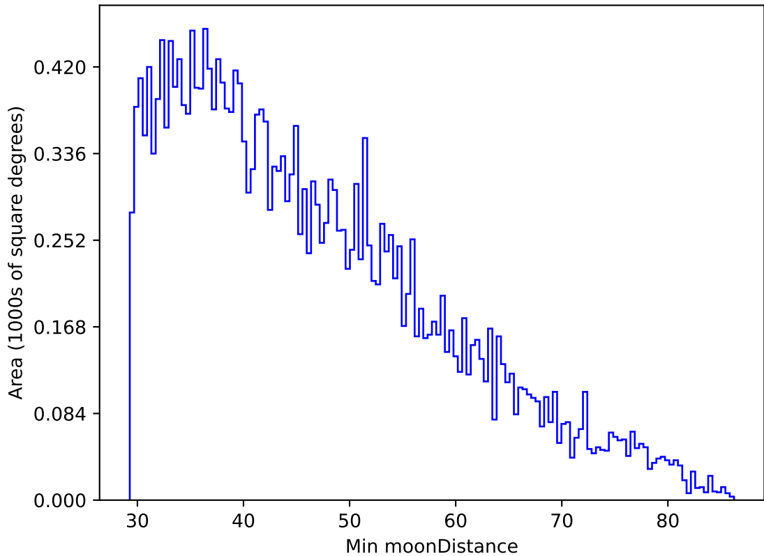
weather_cloudso31v3.4_10yrs All sky g band: Min moonDistance
