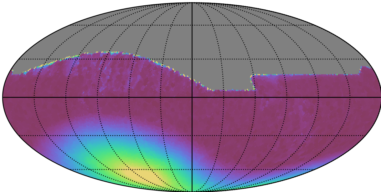
weather_cloudso31v3.4_10yrs All sky all bands: Min moonDistance
