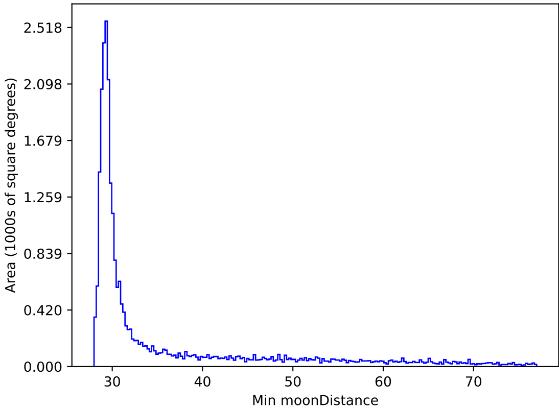
weather_cloudso31v3.4_10yrs All sky all bands: Min moonDistance
