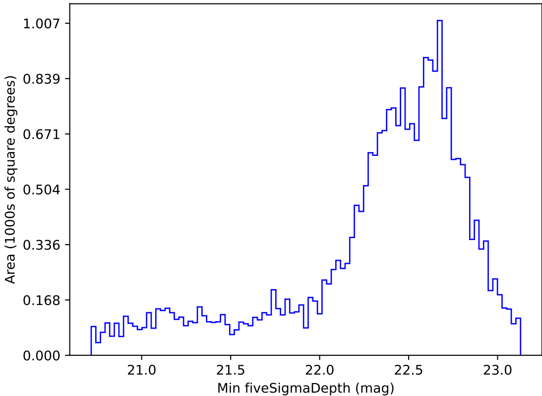
weather_cloudso31v3.4_10yrs Yr 1 z band: Min fiveSigmaDepth
