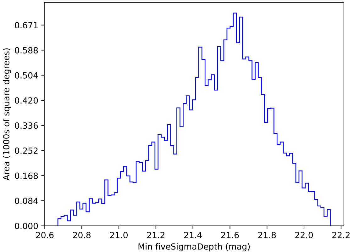
weather_cloudso31v3.4_10yrs Yr 1 y band: Min fiveSigmaDepth
