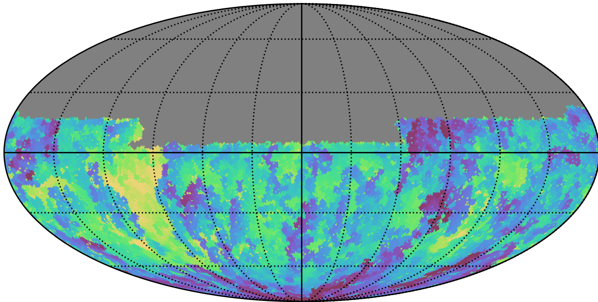
weather_cloudso31v3.4_10yrs Yr 1 u band: Min fiveSigmaDepth
