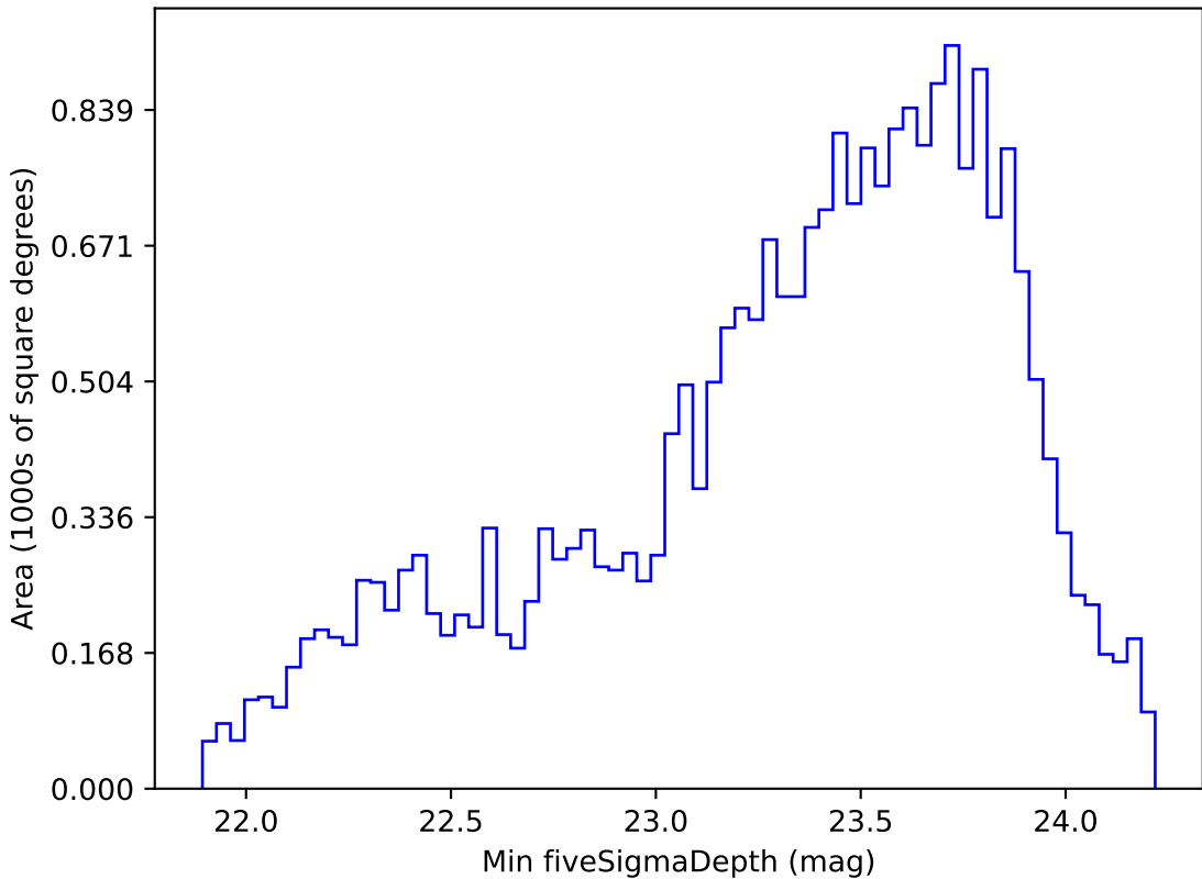
weather_cloudso31v3.4_10yrs Yr 1 r band: Min fiveSigmaDepth
