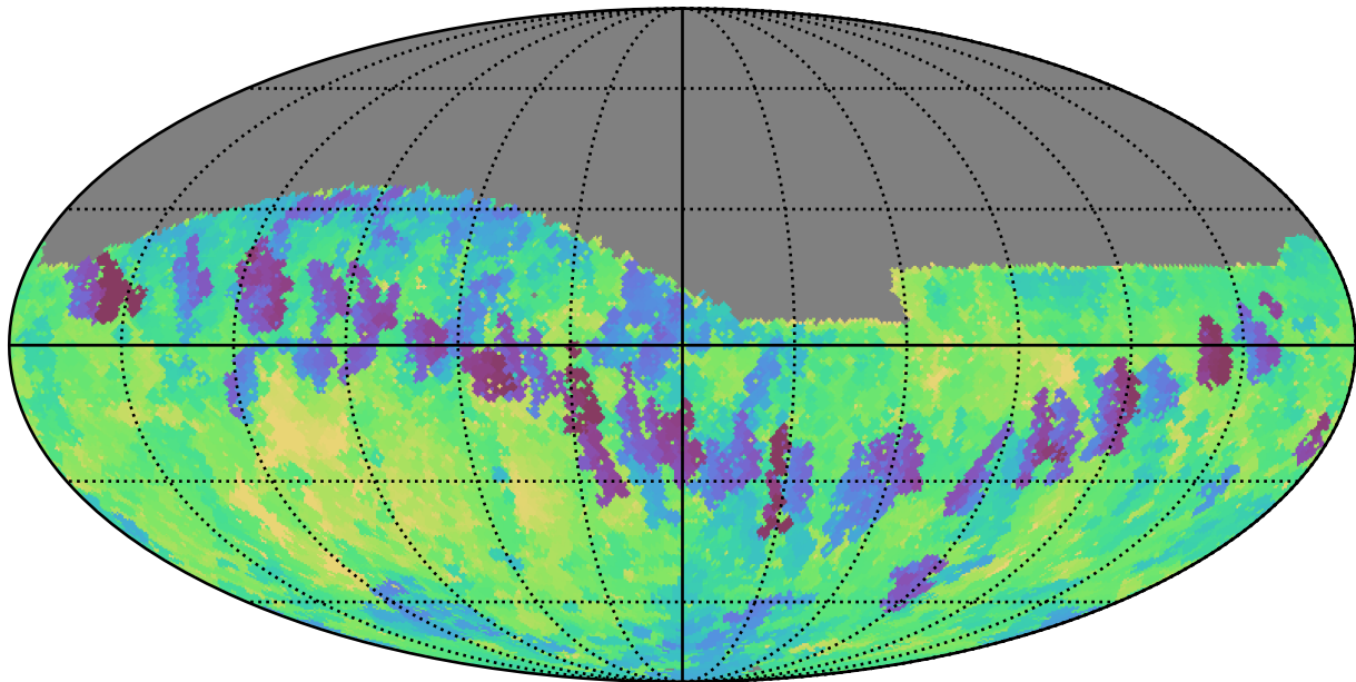
weather_cloudso31v3.4_10yrs Yr 1 i band: Min fiveSigmaDepth
