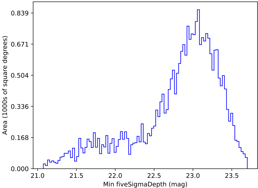
weather_cloudso31v3.4_10yrs Yr 1 i band: Min fiveSigmaDepth
