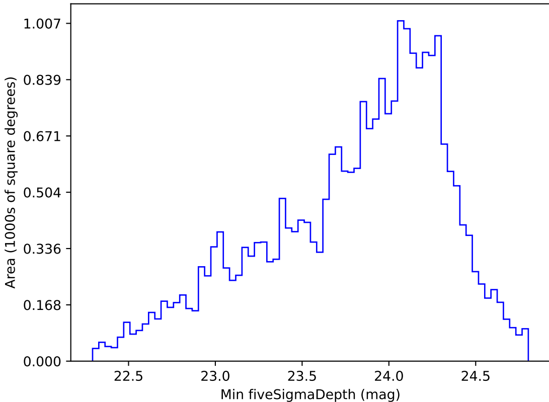
weather_cloudso31v3.4_10yrs Yr 1 g band: Min fiveSigmaDepth
