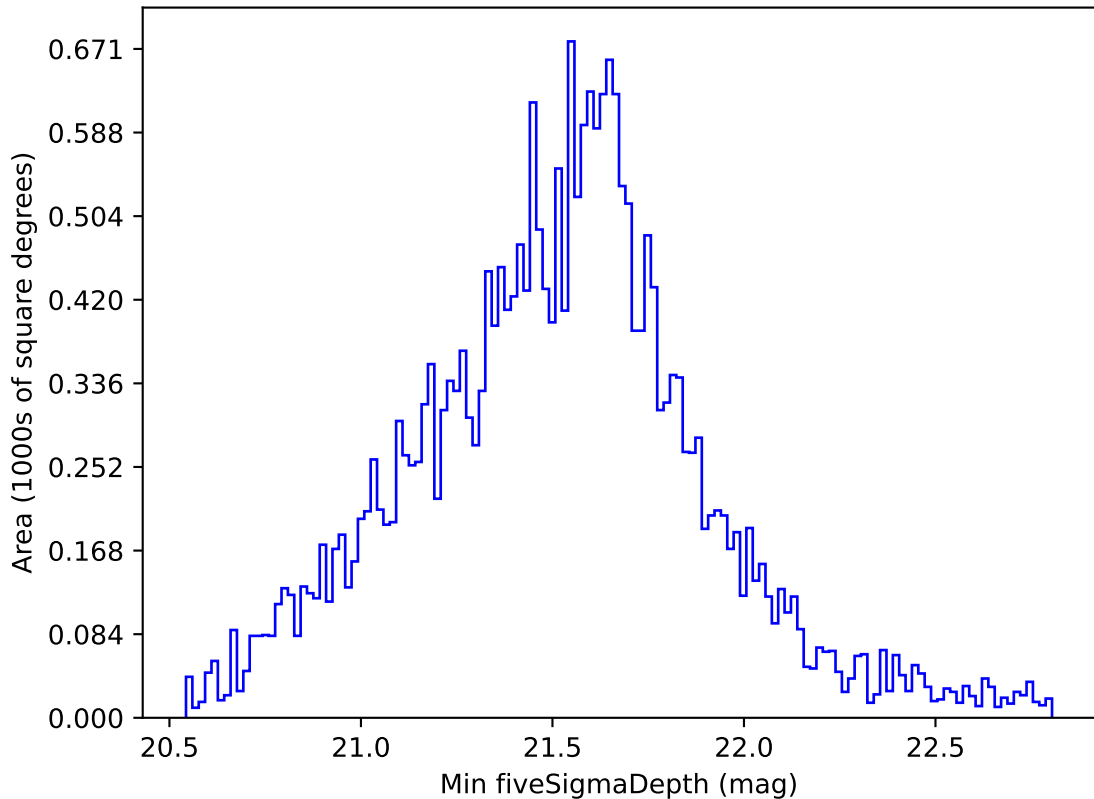
weather_cloudso31v3.4_10yrs Yr 1 all bands: Min fiveSigmaDepth
