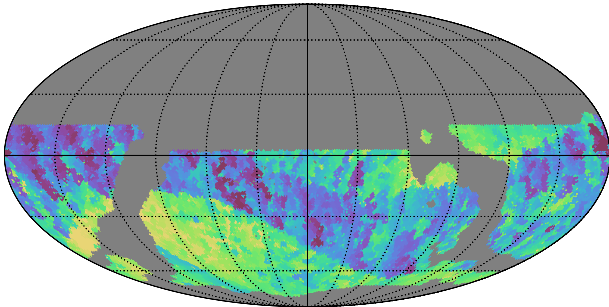
weather_cloudso31v3.4_10yrs WFD z band: Min fiveSigmaDepth
