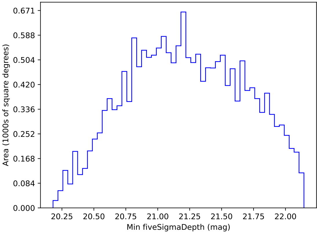
weather_cloudso31v3.4_10yrs WFD z band: Min fiveSigmaDepth
