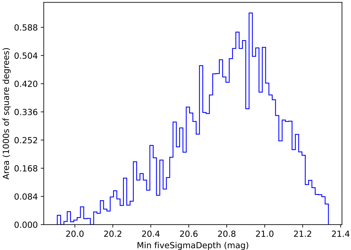
weather_cloudso31v3.4_10yrs WFD y band: Min fiveSigmaDepth
