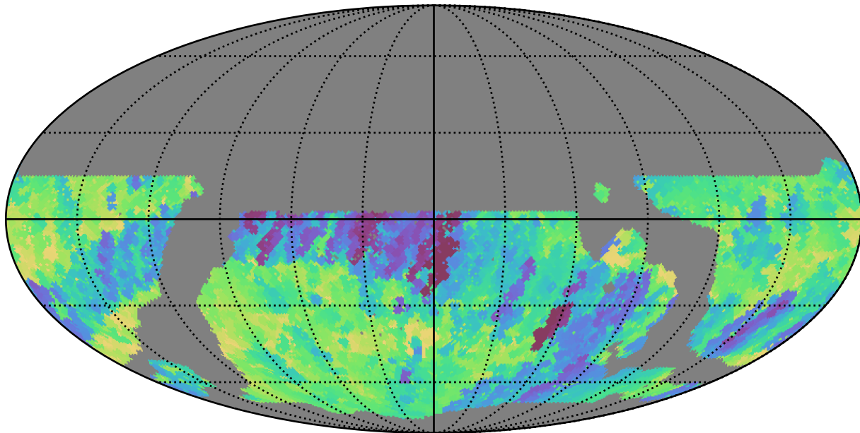
weather_cloudso31v3.4_10yrs WFD r band: Min fiveSigmaDepth
