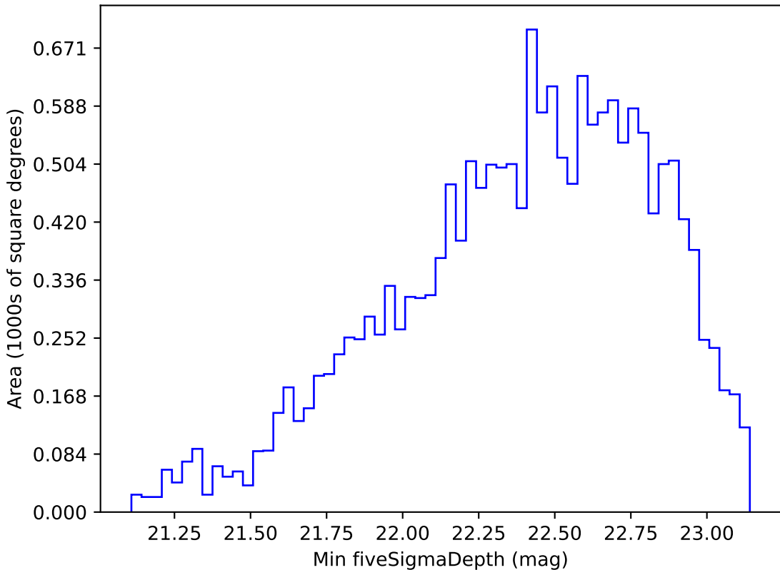
weather_cloudso31v3.4_10yrs WFD r band: Min fiveSigmaDepth
