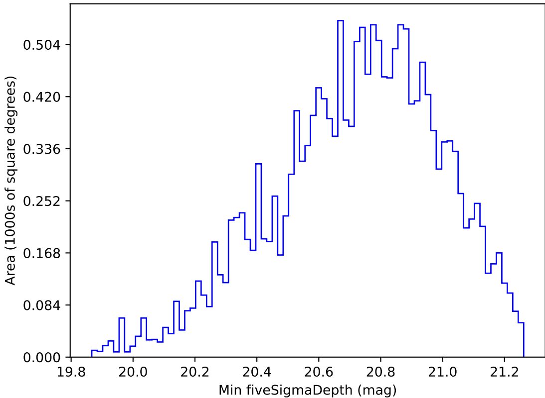
weather_cloudso31v3.4_10yrs WFD all bands: Min fiveSigmaDepth
