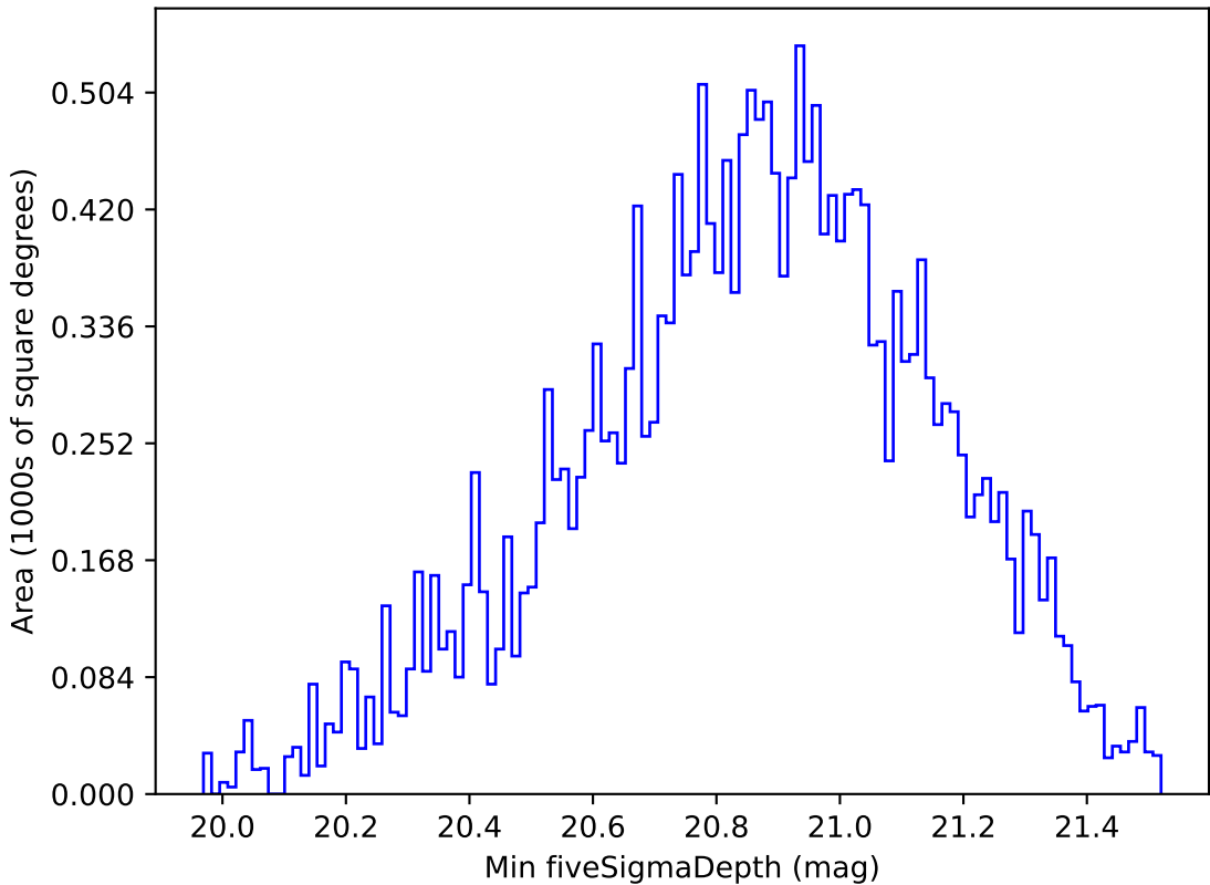
weather_cloudso31v3.4_10yrs All sky y band: Min fiveSigmaDepth
