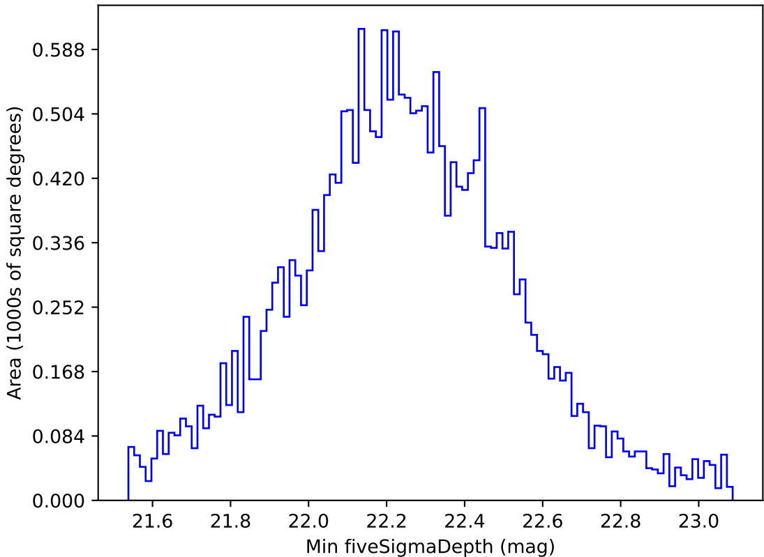
weather_cloudso31v3.4_10yrs All sky u band: Min fiveSigmaDepth
