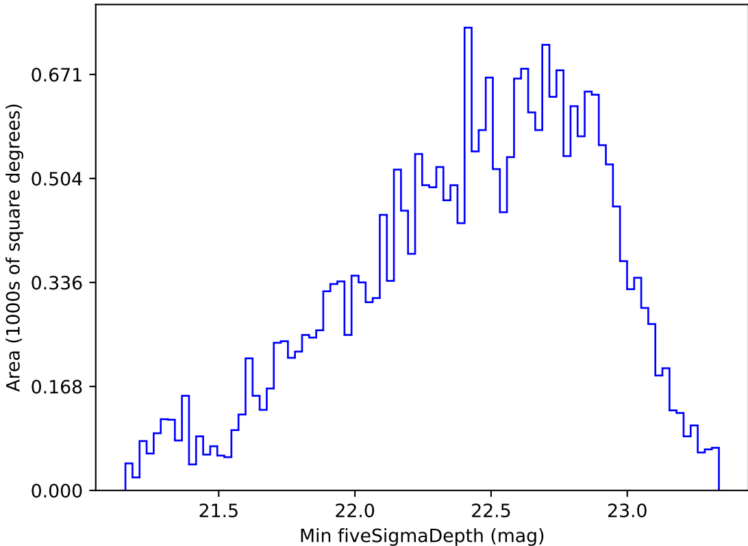
weather_cloudso31v3.4_10yrs All sky r band: Min fiveSigmaDepth
