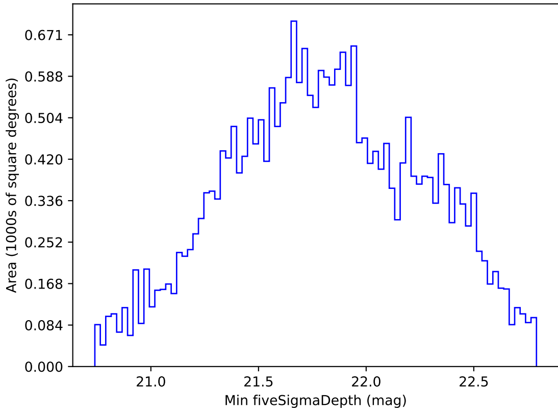
weather_cloudso31v3.4_10yrs All sky i band: Min fiveSigmaDepth
