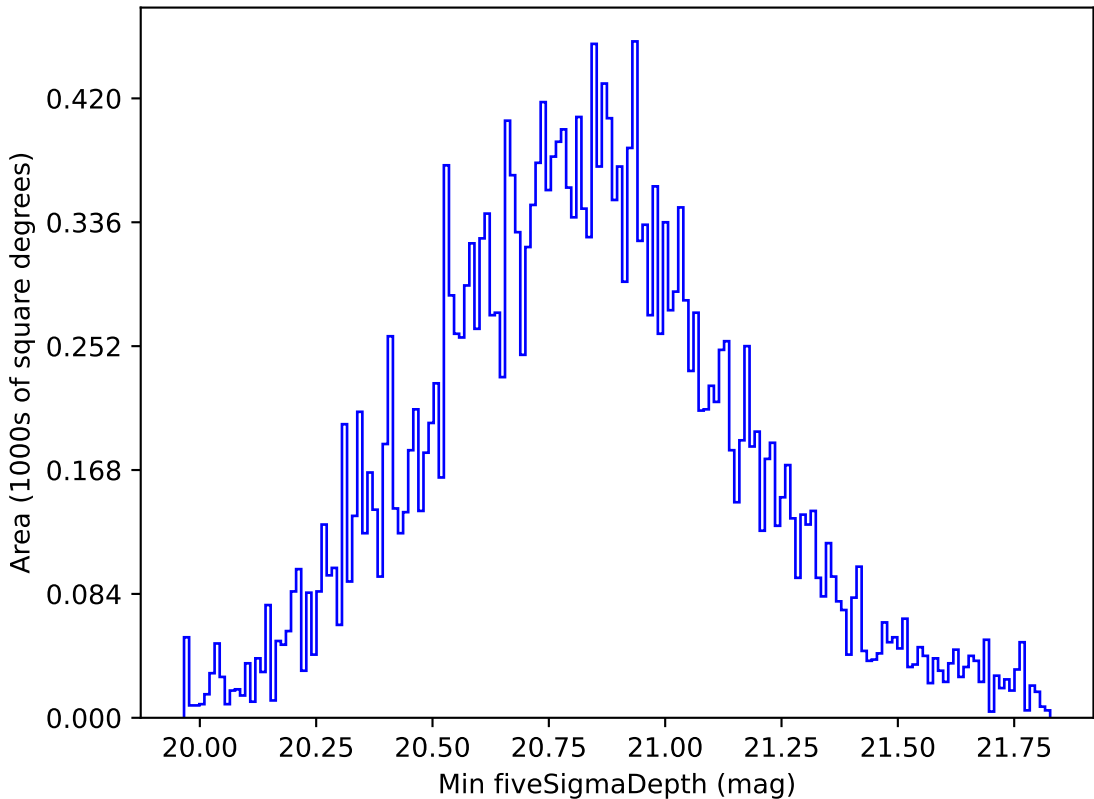
weather_cloudso31v3.4_10yrs All sky all bands: Min fiveSigmaDepth
