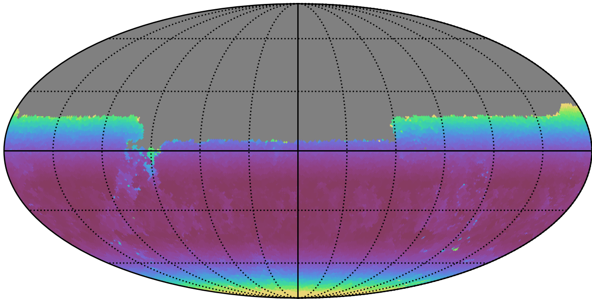
weather_cloudso31v3.4_10yrs Yr 1 y band: Min airmass
