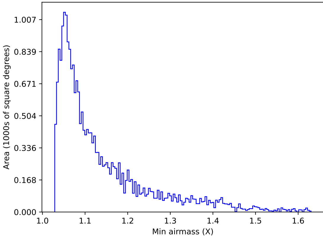
weather_cloudso31v3.4_10yrs Yr 1 u band: Min airmass
