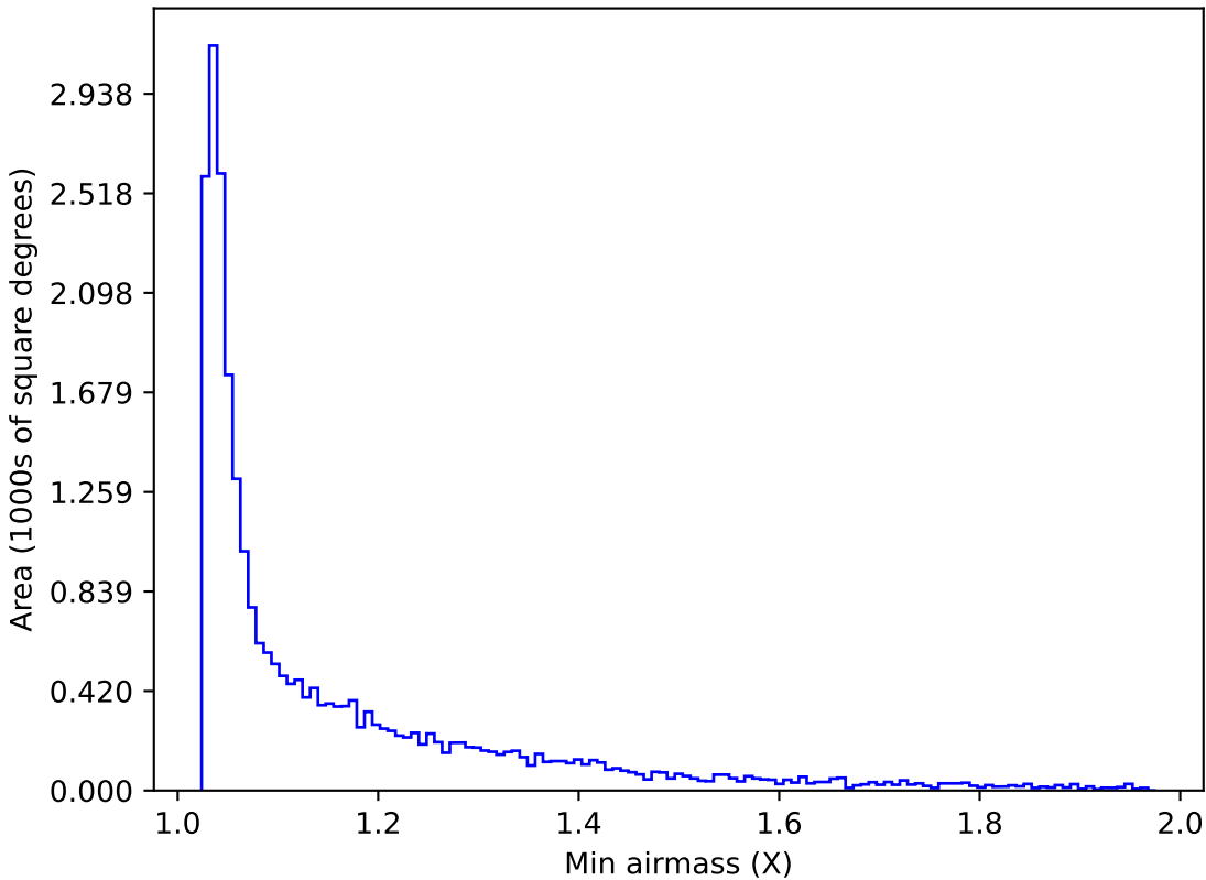
weather_cloudso31v3.4_10yrs Yr 1 r band: Min airmass
