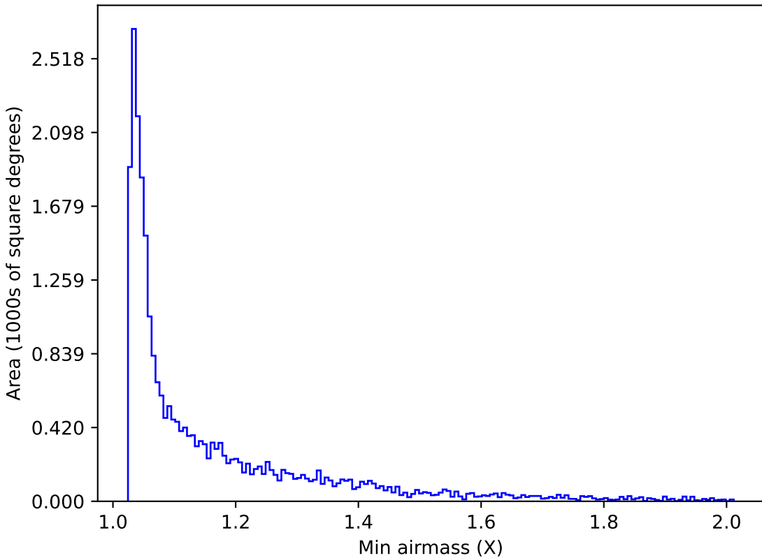
weather_cloudso31v3.4_10yrs Yr 1 i band: Min airmass
