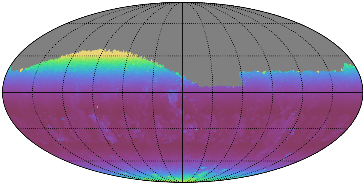
weather_cloudso31v3.4_10yrs Yr 1 g band: Min airmass
